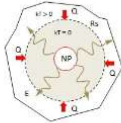
Figure 2. Spherical NP in a Thermal Bath
