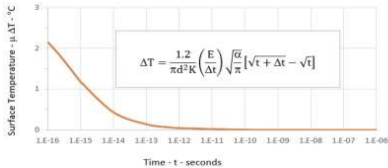
Figure 3. Heat Pulse ( 900 \mu\text{W} ) creating single UVC Photon
