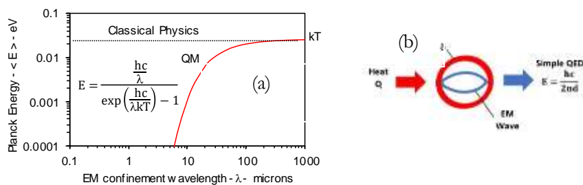
Figure 1. (a) Planck law at 300 K (b) EM heat Q absorption in NP surface
