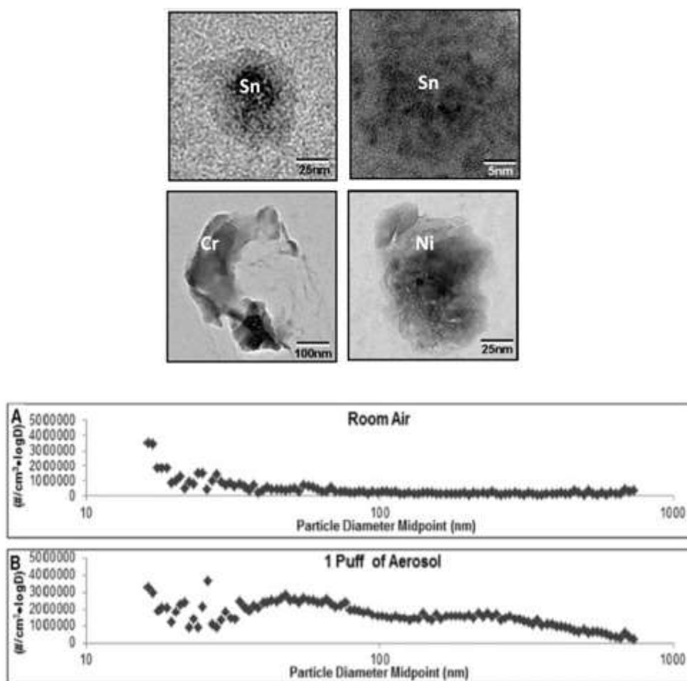
Figure 2. Size and concentration of Sn, Cr, and Ni NPs
