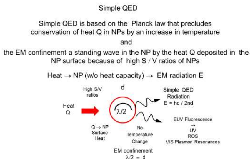
Figure 4. Simple QED conversion of heat to EM radiation
