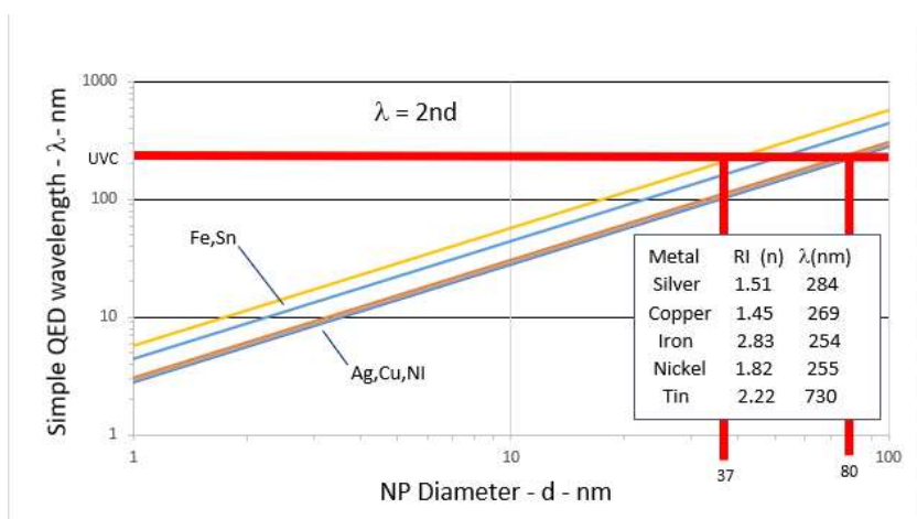
Figure 5. Simple QED wavelength v. NP diameter
