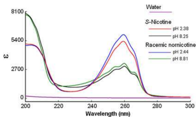
Figure 6. Absorption spectrum of Nicotine.
