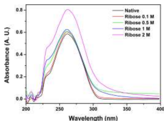
Figure 7. UV absorption spectra of native DNA (black) and glycosylated in D-ribose.
