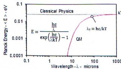
Planck law showing atomic heat capacity vanishes in near-field heat transfer
